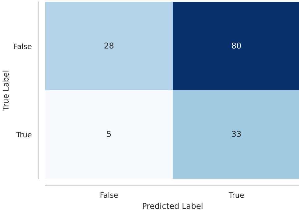
Confusion Matrix - HGB
